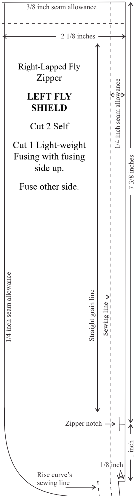
1-28: Caution! Use ONLY as a guide. The fly shield pattern must be drafted from its front pant pattern.
