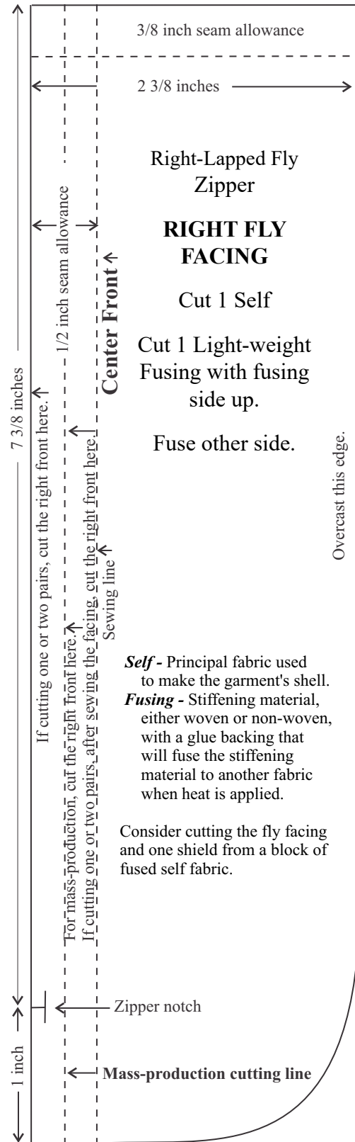
1-29: Caution! Use ONLY as a guide. The fly facing pattern must be drafted from its front pant pattern.
